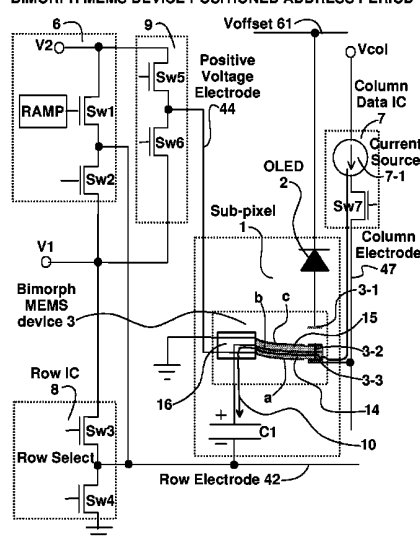
BIMORPH MEMS DEVICE POSITIONED ADDRESS PERIOD
